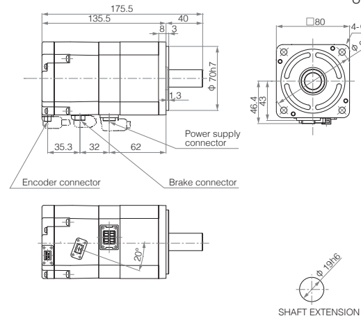
GYB Motor (with brake)
