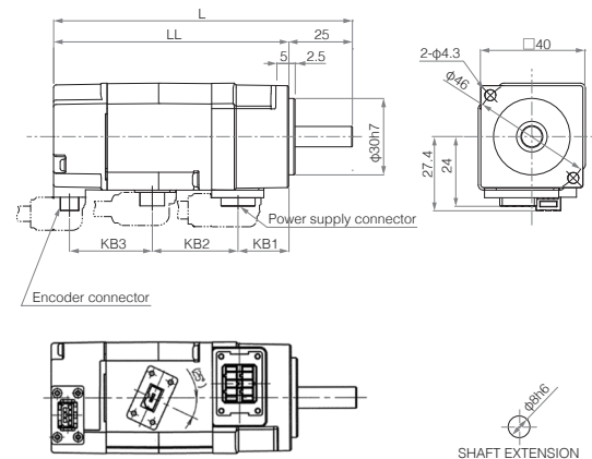
GYB motor (with brake)
