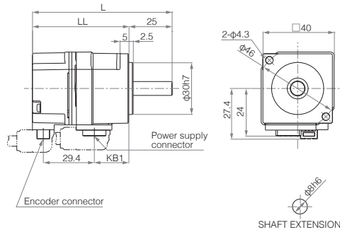
GYB motor (without brake)
