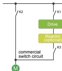
Fig.2 Power system diagram
