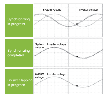
Fig.3 Synchronization/parallel off waveform
