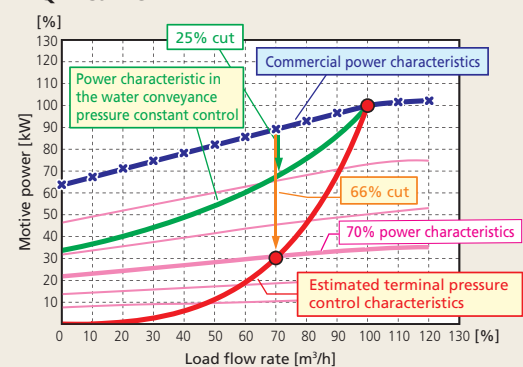
Q-P curve
