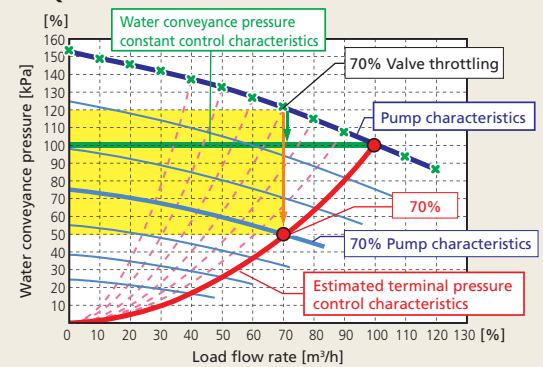
Q-H curve
